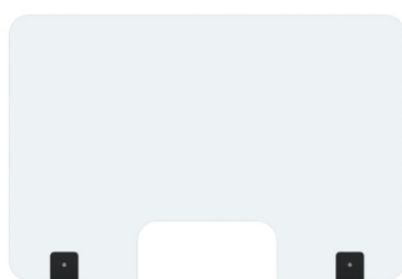
Methacrylate and glass screen 100/120cm Window 35x12cm The over size height is 67,5cm
